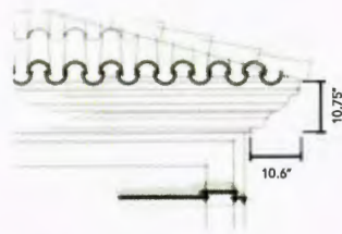
2. EAVE & STONE CORNICE DETAIL AT ENTRY
