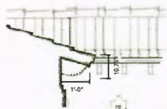
1. RAFTER PROFILE AT COVERED WALK
