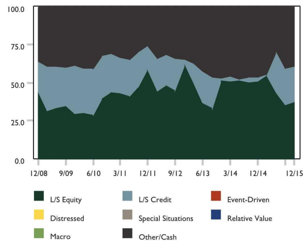
Strategy Weights
