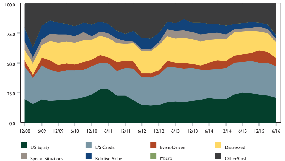
Strategy Weights
